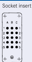
Stamped contacts
